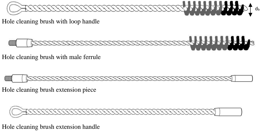
FIGURE 4 – HOLE CLEANING BRUSHES
