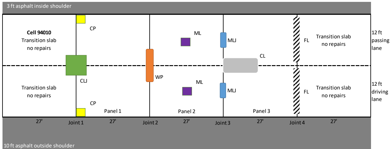
Figure 4.21 Patch Layout for Cell 94010 – Crafc0, Techrete-TBR
