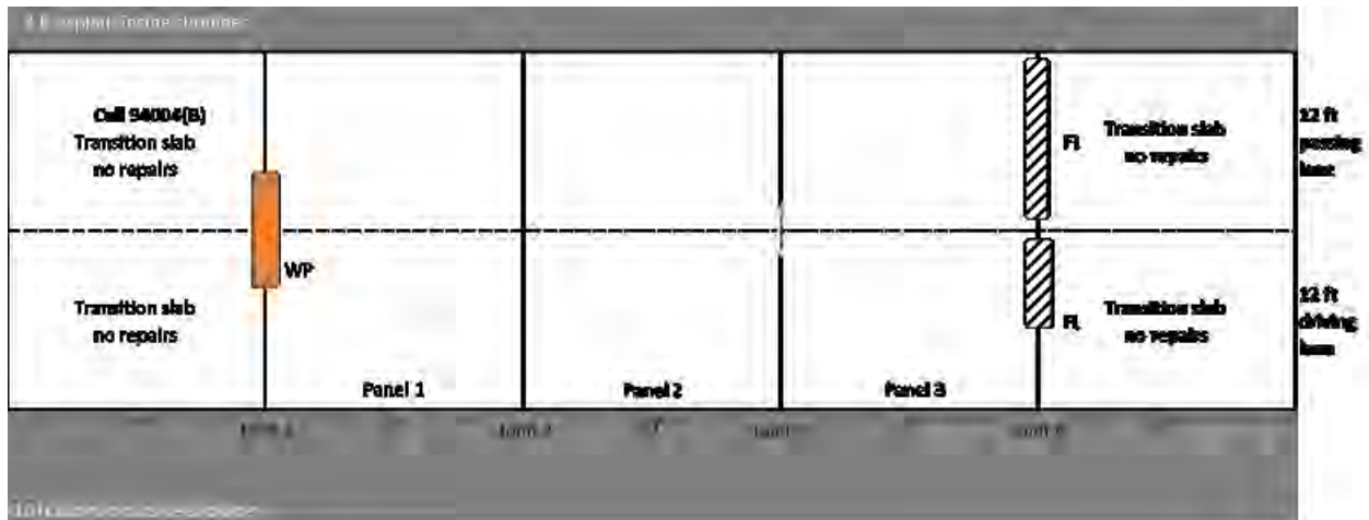
Figure 4.13 Patch Layout for Cell 94004 (B) – Crafc0, HP Concrete Cold Patch
