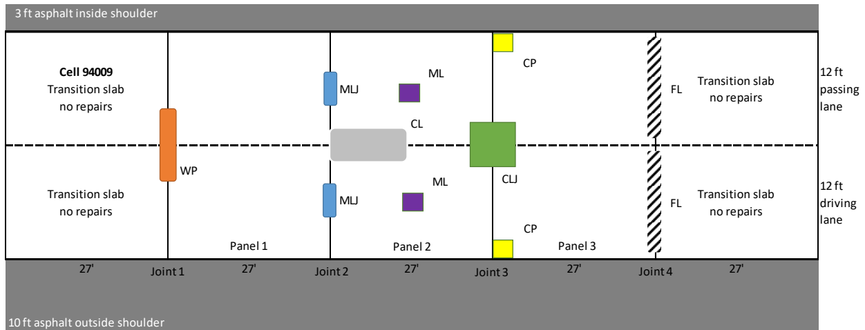
Figure 4.20 Patch Layout for Cell 94009 – Crafco, HP Concrete Cold Patch
